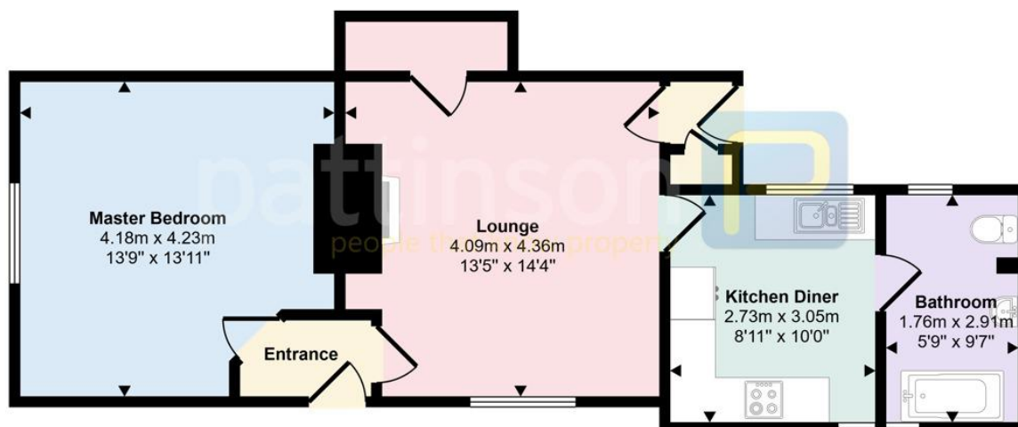
Floorplan
