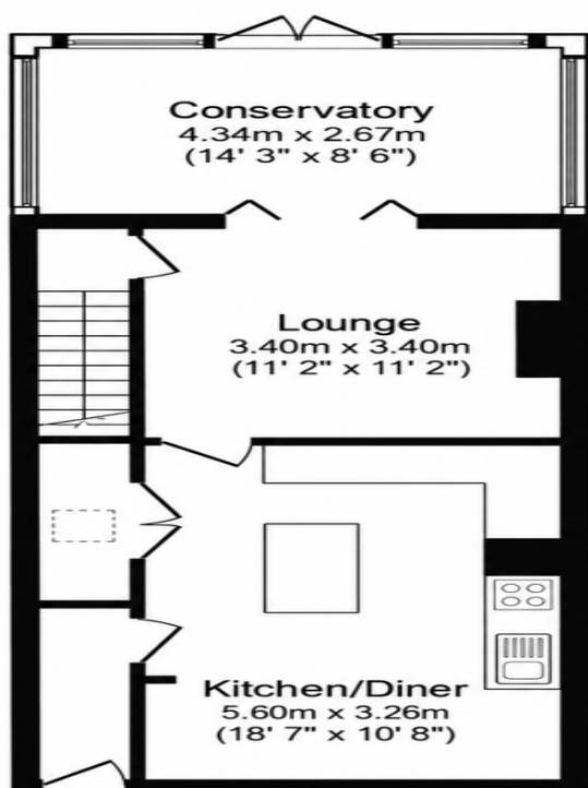
Ground Floor Floor area 51.6 sq.m. (556 sq.ft.)
