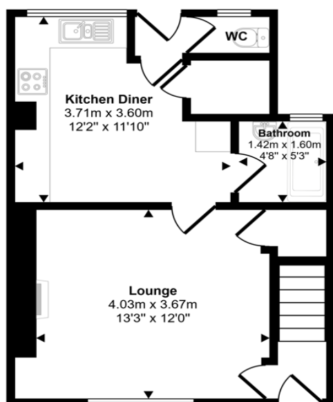
Ground Floor Approx 38 sq m / 408 sq ft
