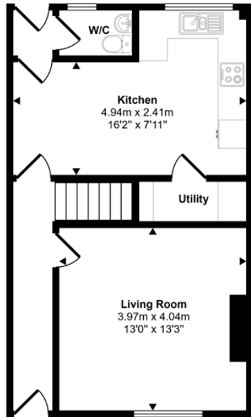
Ground Floor Approx 43 sq m / 458 sq ft
