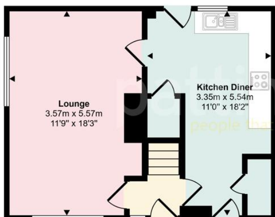
Ground Floor Approx 39 sq m / 421 sq ft
