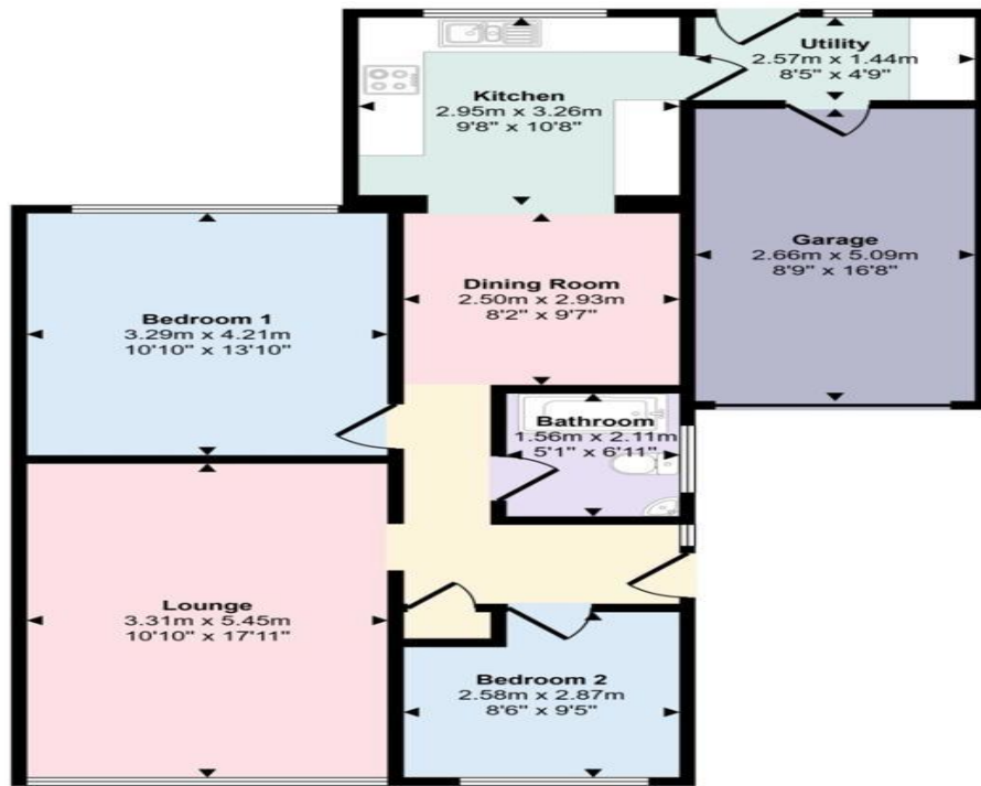
Floorplan
