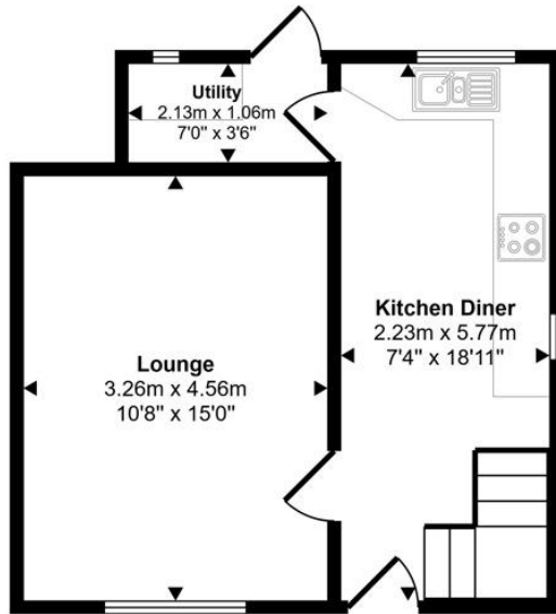
Ground Floor Approx 31 sq m / 336 sq ft
