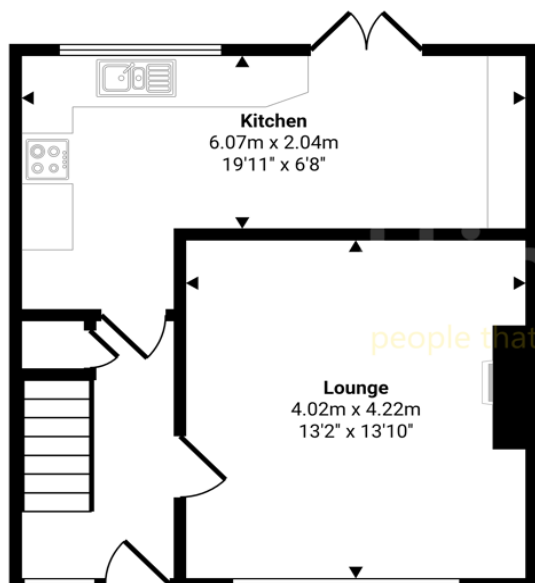
Ground Floor Approx 39 sq m / 419 sq ft
