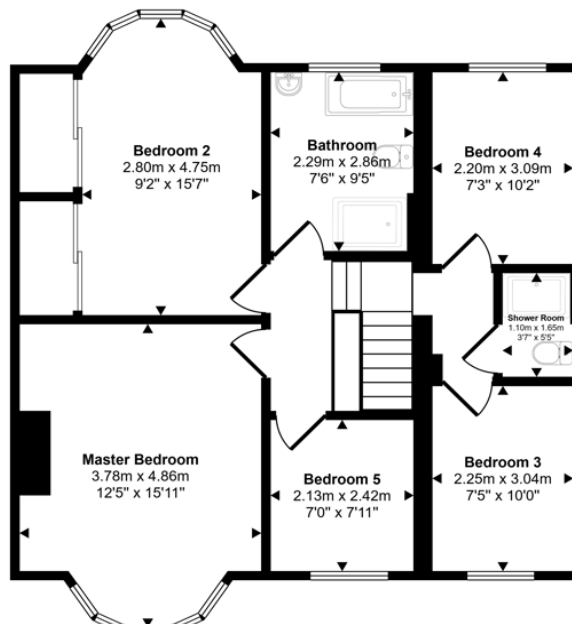
First Floor Approx 73 sq m / 786 sq ft
