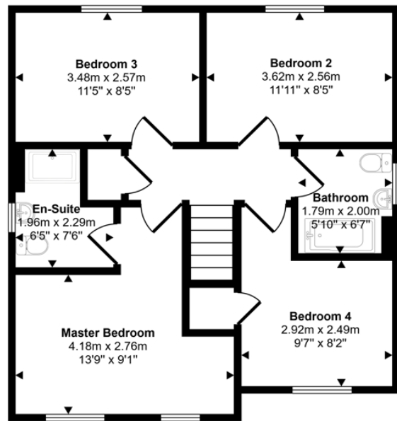
First Floor Approx 56 sq m / 599 sq ft
