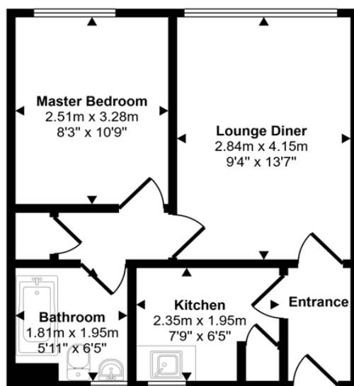
Floorplan
