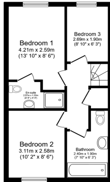
First Floor Floor area 38.3 sq.m. (412 sq.ft.)
