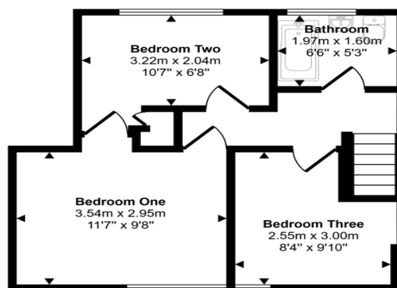
First Floor Approx 35 sq m / 380 sq ft
