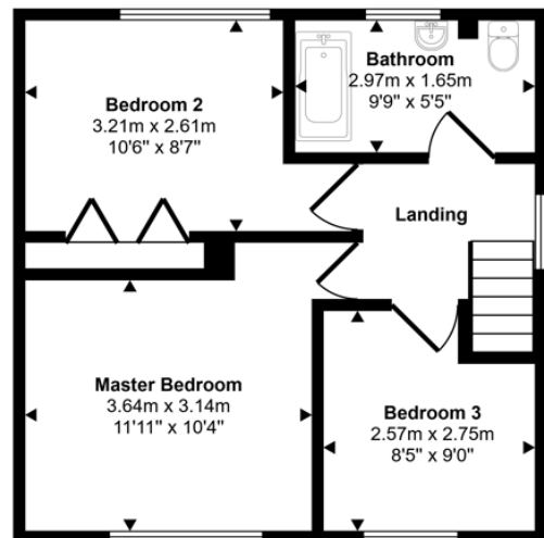
First Floor Approx 41 sq m / 437 sq ft
