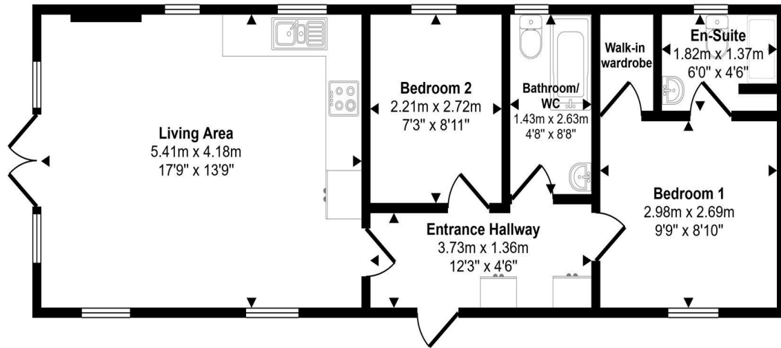
Floorplan
