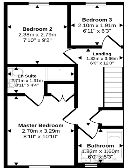
First Floor Approx 36 sq m / 383 sq ft
