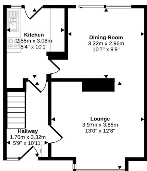
Ground Floor Approx 39 sq m / 423 sq ft
