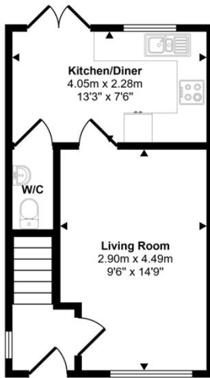
Ground Floor Approx 28 sq m / 299 sq ft
