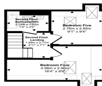
Second Floor Approx 31 sq m / 331 sq ft
