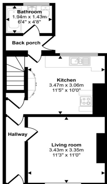
Ground Floor Approx 34 sq m / 366 sq ft
