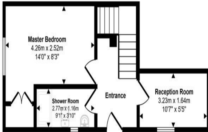
Ground Floor Approx 29 sq m / 316 sq ft
