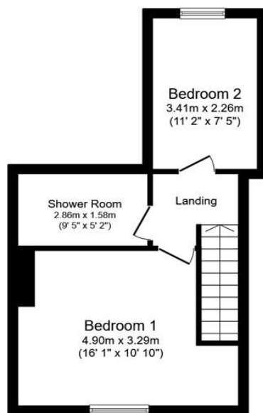
First Floor Floor area 32.7 sq.m. (352 sq.ft.)
