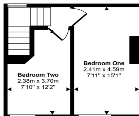
First Floor Approx 23 sq m / 246 sq ft
