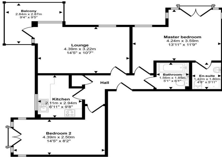
Floorplan
