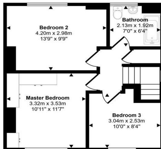
First Floor Approx 43 sq m / 467 sq ft
