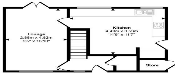
Ground Floor Approx 36 sq m / 390 sq ft
