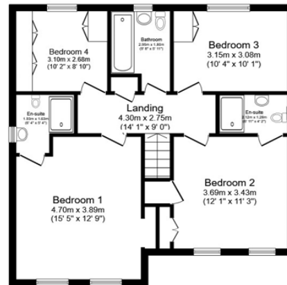
First Floor Floor area 69.9 sq.m. (752 sq.ft.)
