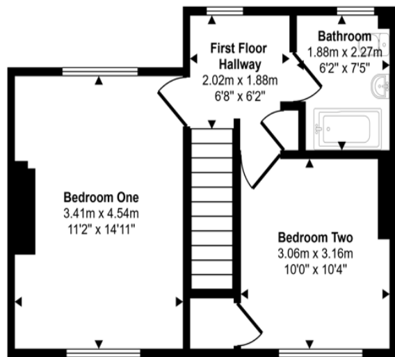
First Floor Approx 39 sq m / 418 sq ft
