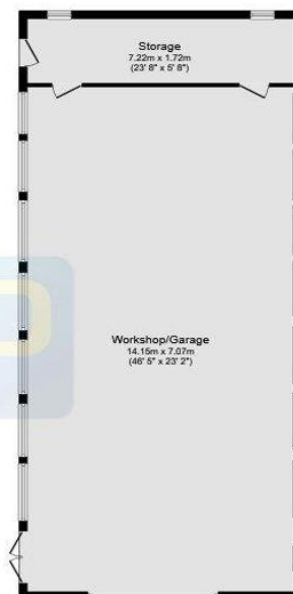
Outbuilding
