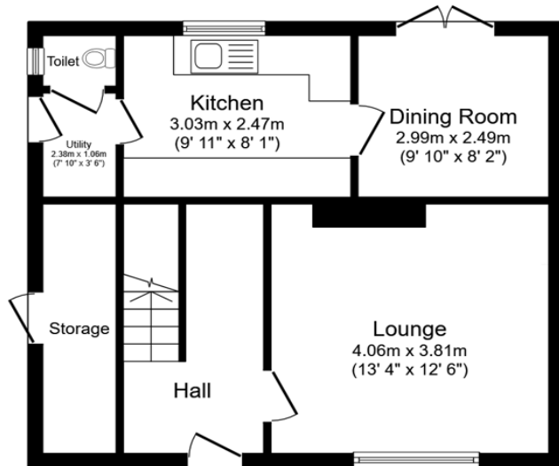
Ground Floor Floor area 46.5 sq.m. (500 sq.ft.)
