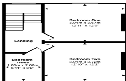
First Floor Approx 44 sq m / 476 sq ft
