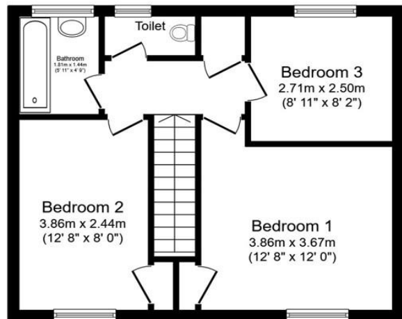
First Floor Floor area 42.4 sq.m. (457 sq.ft.)
