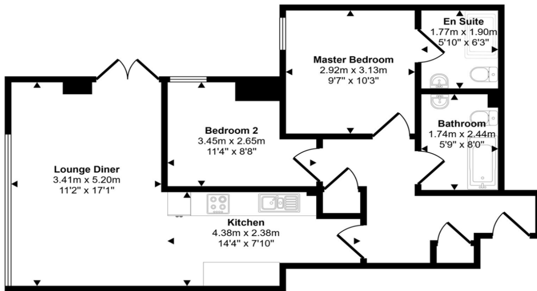
Floorplan
