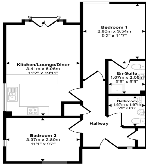
Floorplan
