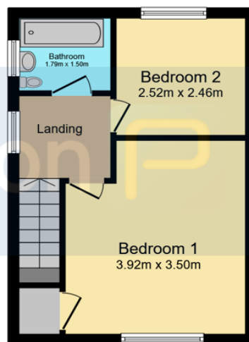
First Floor Floor area 28.8 sq.m.
